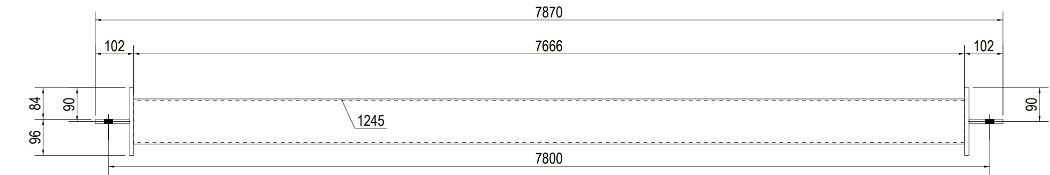
FRONT VIEW
